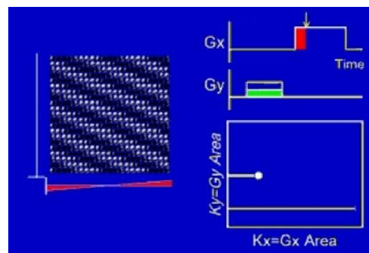
Figure 30. Creating stripe patterns in arbitrary directions with the sequential application of G_y and G_x gradients. A K-space plot traces out the area of the G_x and G_y gradient for the K_x and K_y locations respectively.
